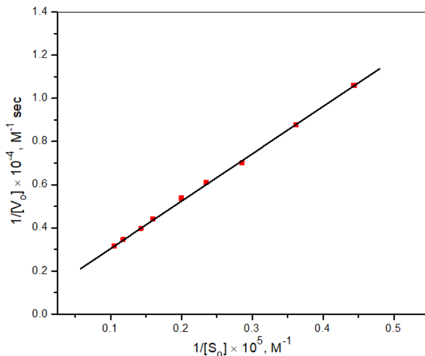
Figure 3. The Lineweaver-Burk plot at constant [Pd^{2+}] in the absence of ALA at [Pyrazine] = 3.0 \times 10^{-4} mole L^{-1} , pH = 4.0 \pm 0.02 , Temp = 318 \pm 0.1 K, I = 0.10 mole L^{-1} ( NaClO_4 ), [Pd(II)] = 6.0 \times 10^{-4} mole L^{-1} , and [SLS] = 8.5 \times 10^{-3} mole L^{-1}
