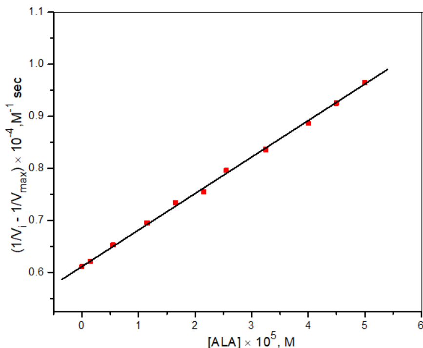
Figure 4. The plot of (1/V_i - 1/V_{max}) versus initial [ALA] at [Pyrazine] = 3.0 \times 10^{-4} mole L -1 , pH = 4.0 \pm 0.02 , Temp = 318 \pm 0.1 K, [Ru(CN) 6 4- ] = 2.75 \times 10^{-5} mole L -1 , I = 0.10 mole L -1 (NaClO 4 ), [Pd(II)] = 6.0 \times 10^{-4} mole L -1 , and [SLS] = 8.5 \times 10^{-3} mole L -1
