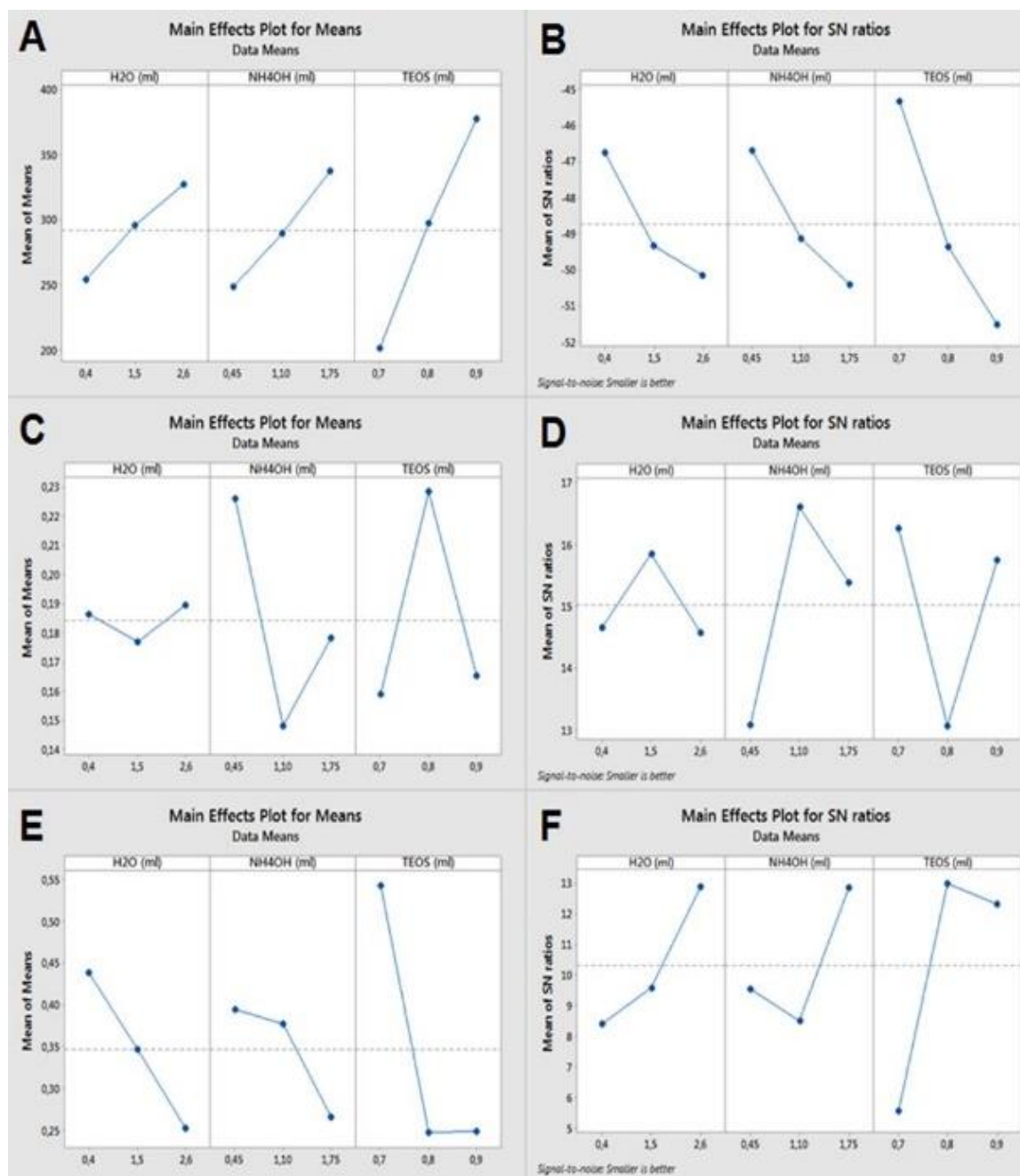
Figure 1. The main effect plots for the smallest particle size: A and B belong to the average particle size, and C and D belong to the optimization made according to the polydispersity index. E and F are obtained with TOPSIS-based Taguchi design.
