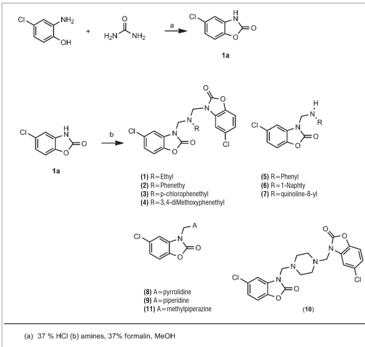
FIGURE 1. Synthesis of the compounds 1-11.
